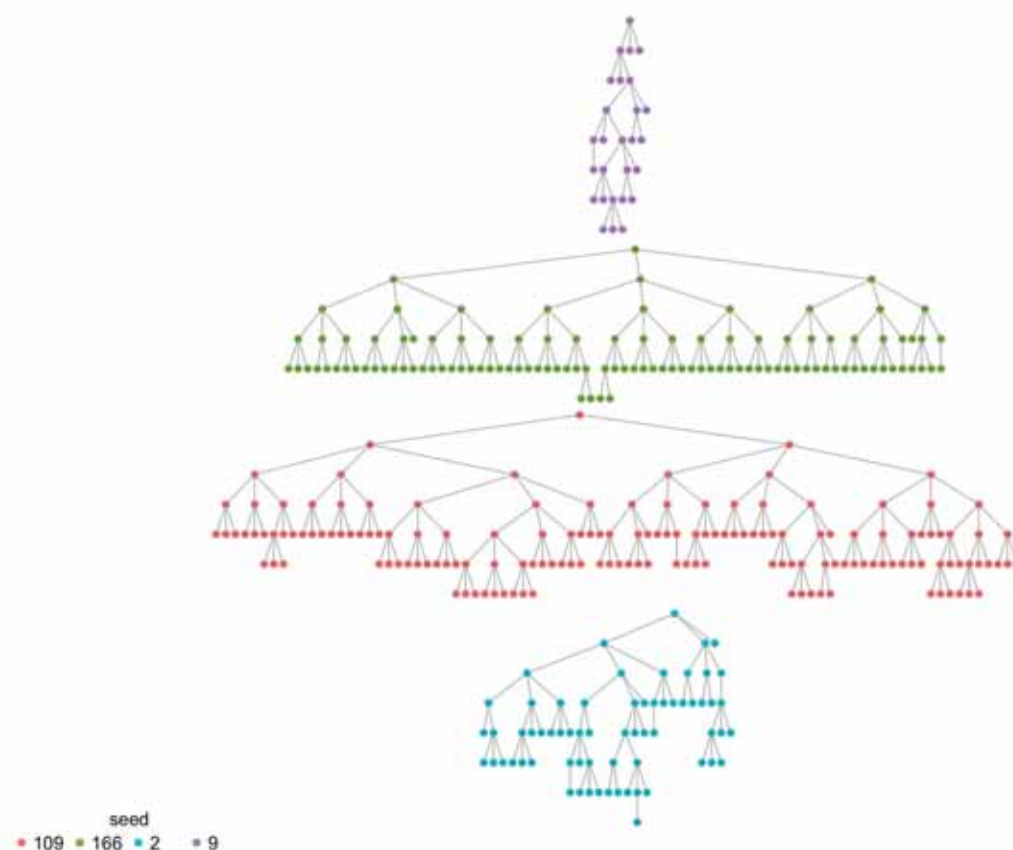
Figure 6. Recruitment tree – FSW Galle
