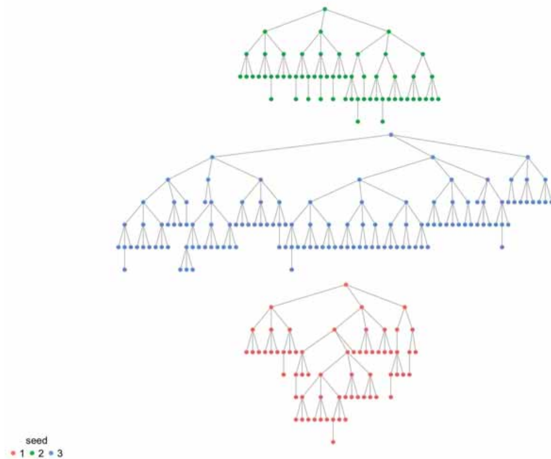
Figure 20. Recruitment tree – TGW Colombo
