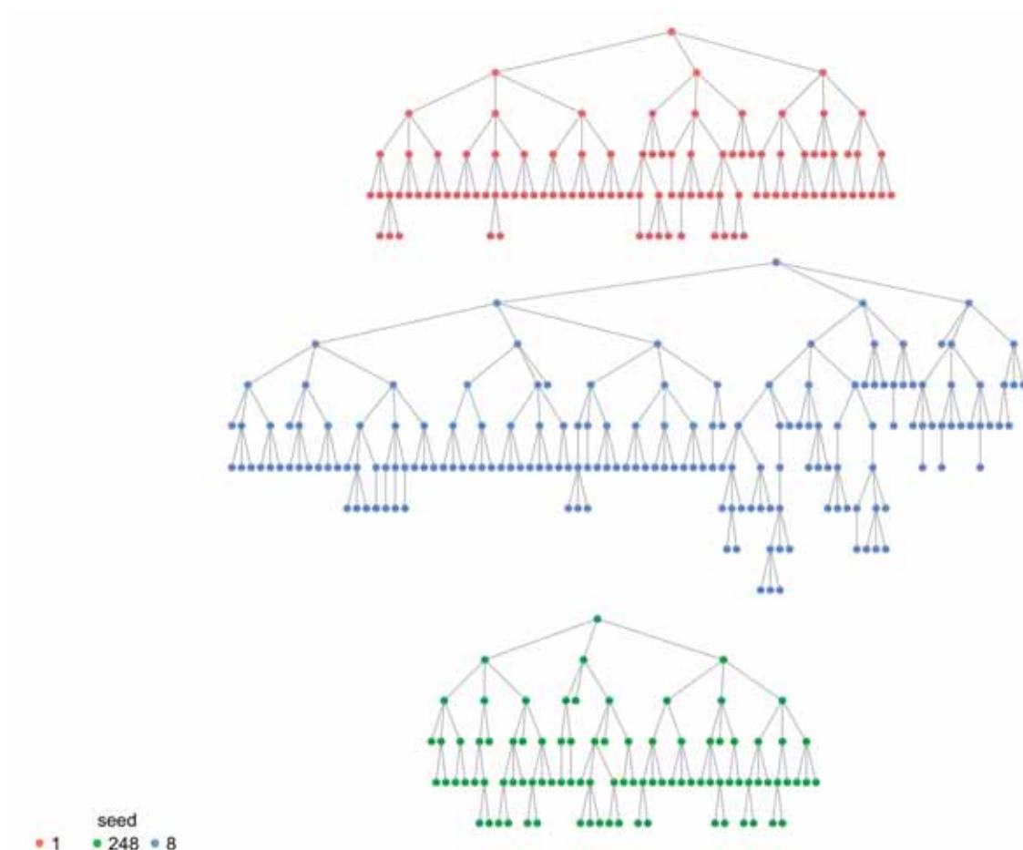
Figure 18. Recruitment tree - BB
